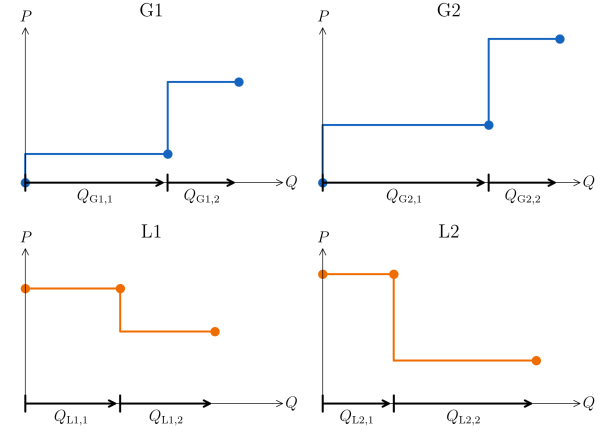
Figure 13: Reformulating the optimization problem of Example 4 with one decision variable for each step in the generators' and loads' supply and demand "staircases".
