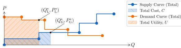
Figure 9: Determining the market-clearing prices and quantities for the two-node grid of Example 3 with a congested 8-MW line.
