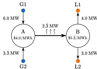
Figure 7: Network of Example 3.
