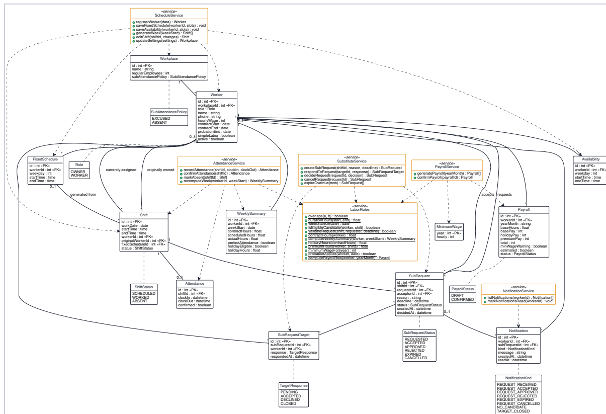
Figure 7. Analysis class diagram (domain view)
