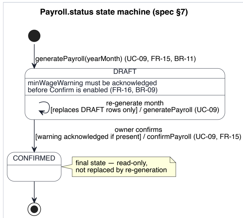
Figure 6. State machine diagram of Payroll
