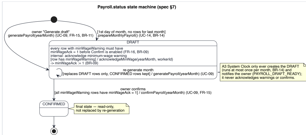
Figure 17. State machine of Payroll.status
