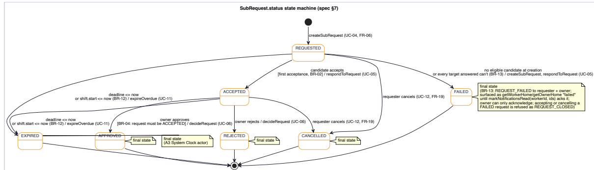
Figure 15. State machine of SubRequest.status
