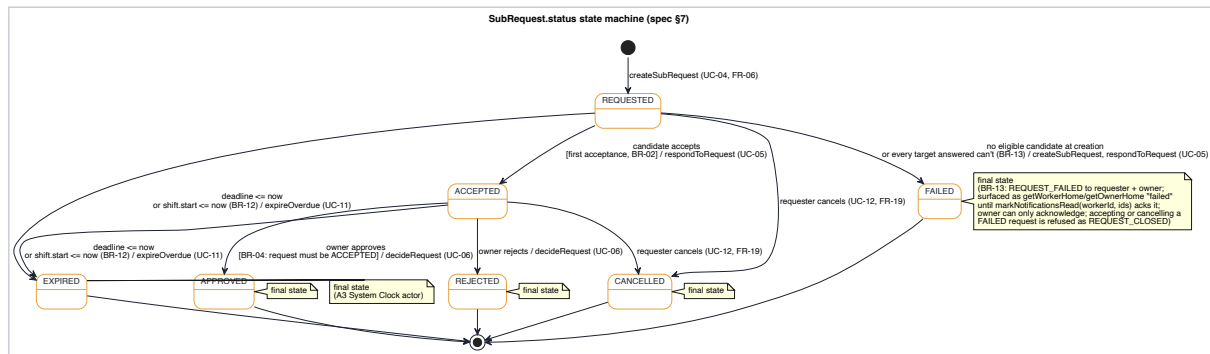
Figure 5. State machine diagram of a substitute request (SubRequest.status)
