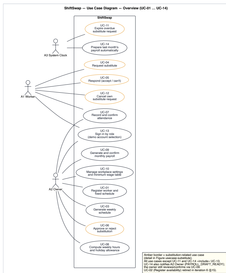
Figure 2. Use-case diagram of ShiftSwap (UML 2.5)
