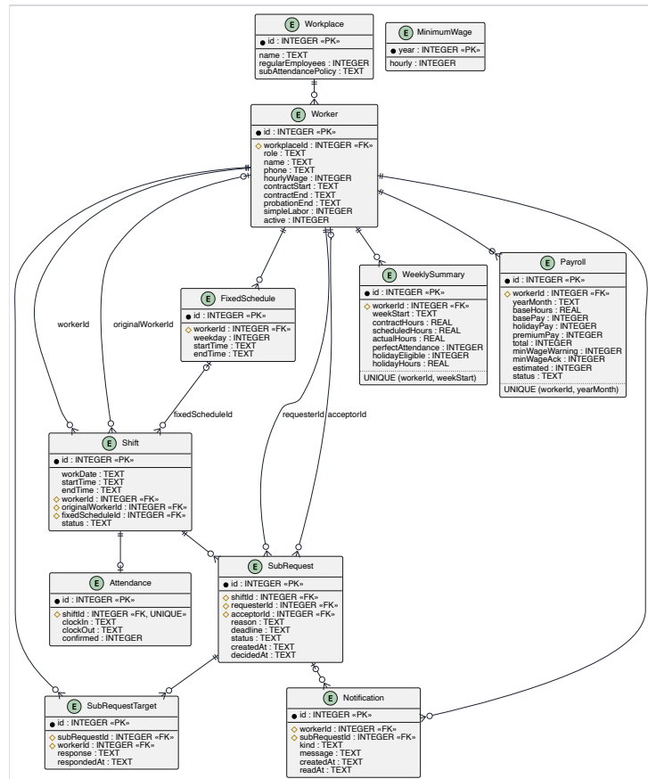
Figure 9. Entity-relationship diagram of the ShiftSwap database (11 tables)
