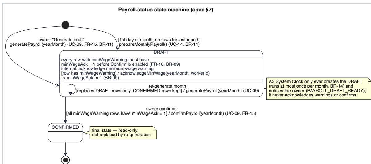
Figure 6. State machine diagram of Payroll
