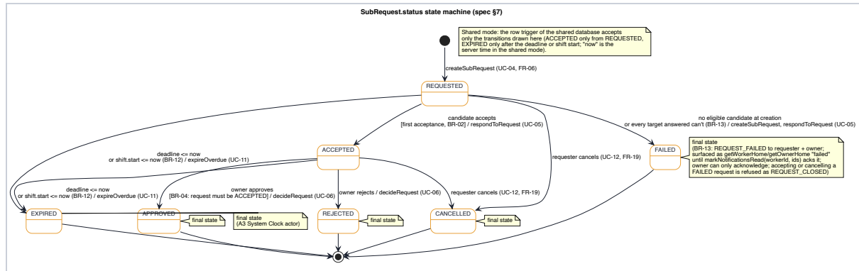
Figure 4. State machine diagram of SubRequest
