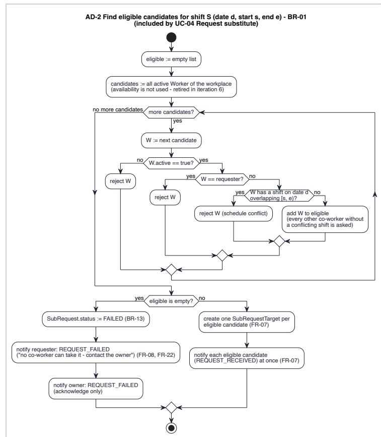
Figure 2. Activity diagram AD-2: candidate selection (BR-01)
