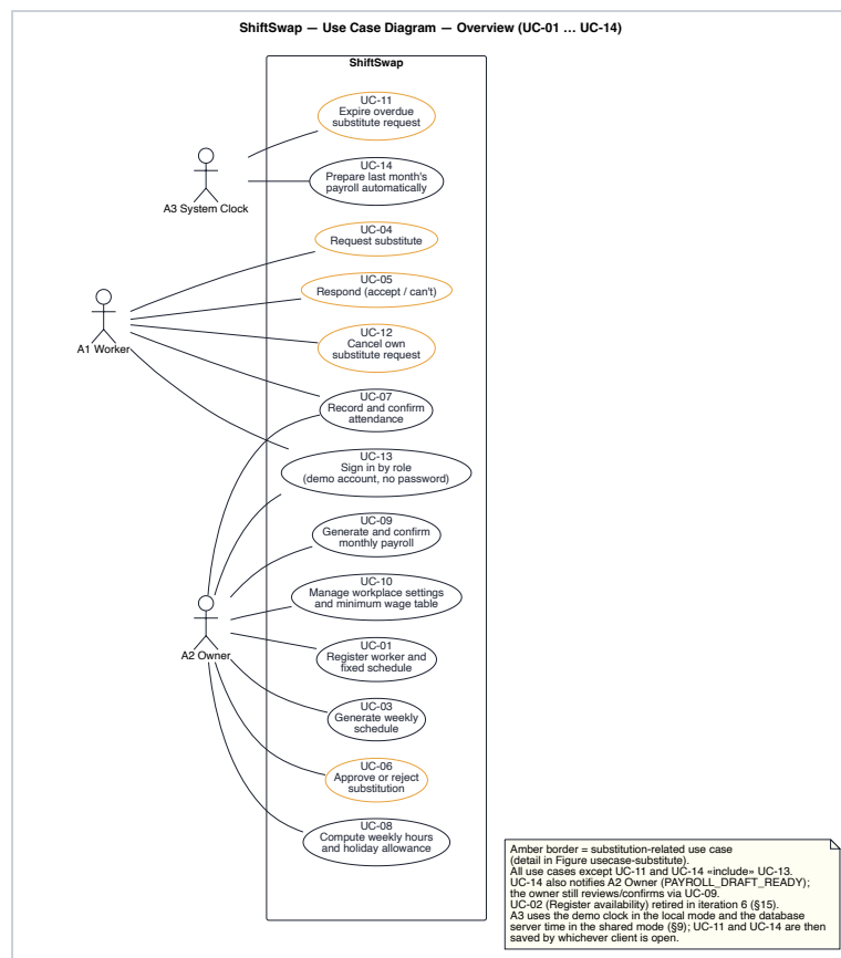
Figure 1. Use case diagram of ShiftSwap
