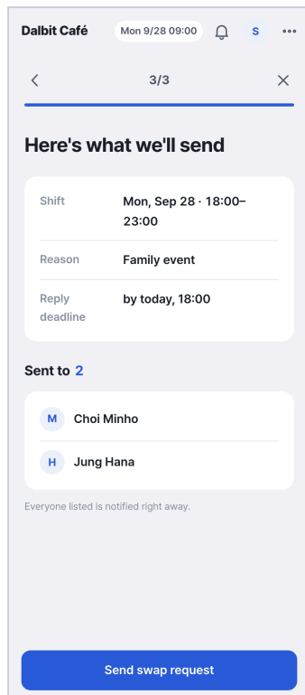
Figure 11. Request substitute, step 3 of 3 (UC-04), Lee Seoyeon. "Here's what we'll send": shift Mon, Sep 28 18:00–23:00, reason "Family event", reply deadline "by today, 18:00" (the shift start, earlier than now + 24 h). "Sent to 2": Choi Minho and Jung Hana. Button: Send swap request .
