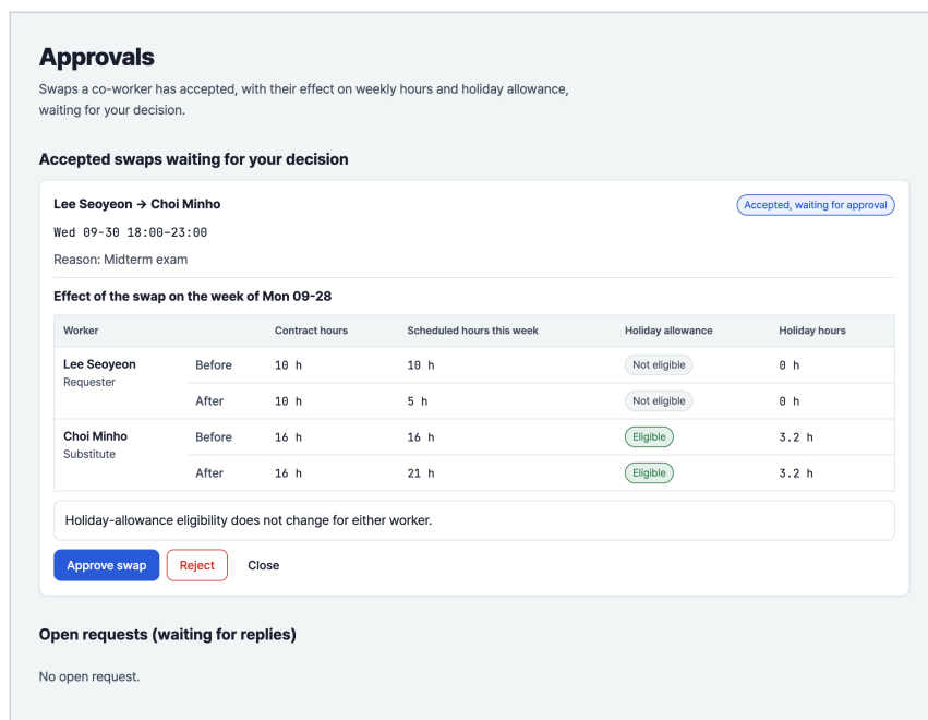
Figure 15. Approval panel (UC-06, FR-11). Lee Seoyeon → Choi Minho for Wed 09-30 18:00–23:00, “Accepted, waiting for approval”. For the week of Mon 09-28, Seoyeon keeps 10 contract hours, her scheduled hours fall from 10 to 5 h, and she is not eligible before or after (0 h). Minho keeps 16 contract hours, his scheduled hours rise from 16 to 21 h, and he is eligible before and after with 3.2 holiday hours. The note reads “Holiday-allowance eligibility does not change for either worker.” Buttons: Approve swap , Reject , Close .
