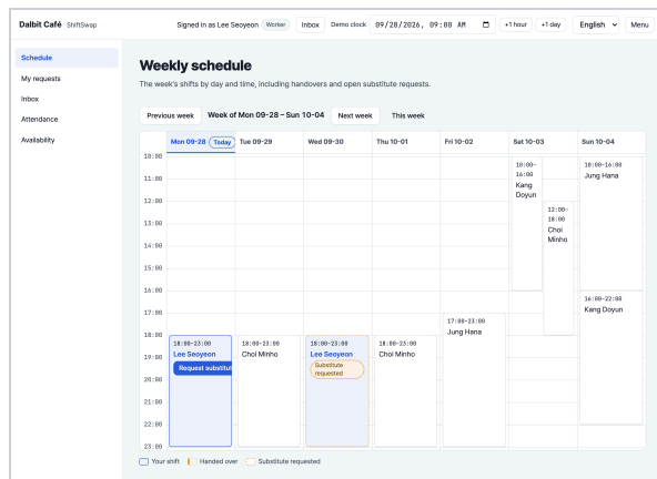
Figure 13. Weekly board, worker view (UC-03, UC-04), signed in as Lee Seoyeon. Her own shifts (Mon and Wed 18:00–23:00) are shaded blue with her name in blue. The Monday shift offers Request substitute ; the Wednesday shift already carries “Substitute requested”. The worker menu has Schedule, My requests, Inbox, Attendance and Availability, and no editing controls.
