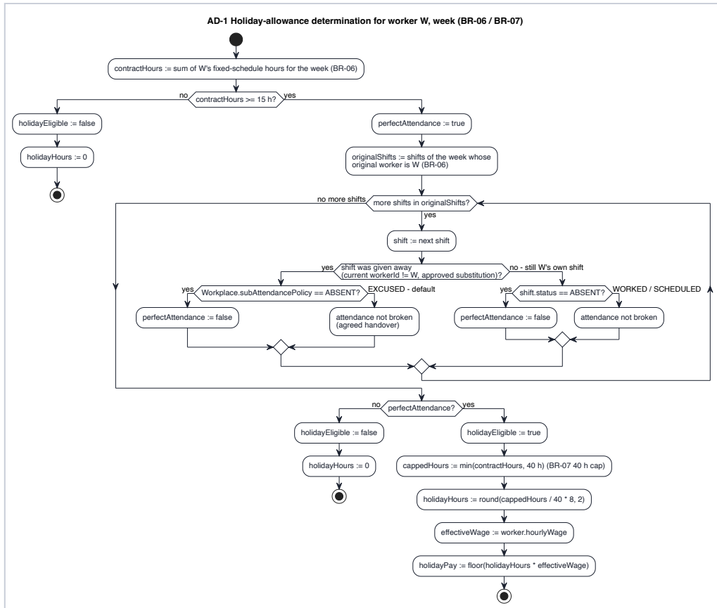
Figure 3. Activity diagram AD-1: holiday-allowance determination (BR-06, BR-07)
