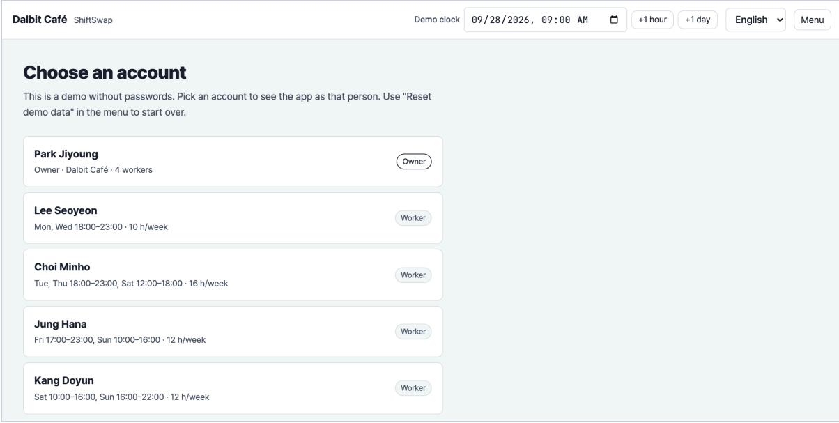
Figure 8. Sign-in (UC-13). “Choose an account” lists Park Jiyoung (Owner, Dalbit Café, 4 workers) and the four workers with their fixed shifts and weekly hours: Lee Seoyeon 10 h, Choi Minhho 16 h, Jung Hana 12 h, Kang Doyun 12 h. A note says the demo has no passwords. The header shows the demo clock at 09/28/2026 09:00 with +1 hour and +1 day, the language switch and the menu.
