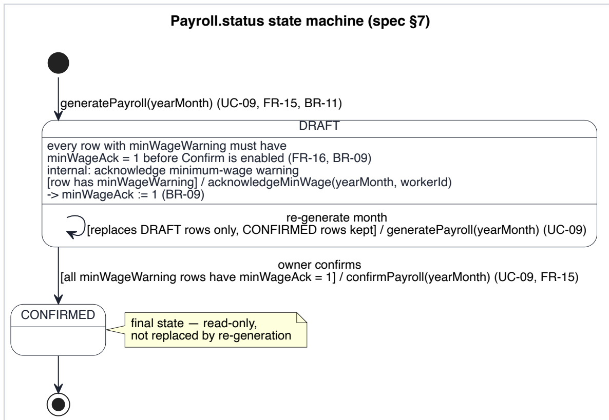
Figure 6. State machine diagram of Payroll
