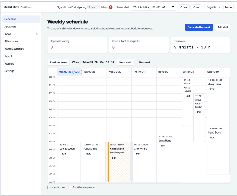
Figure 16. Weekly board after approval (UC-06, BR-04). The Wednesday 09-30 18:00–23:00 shift now shows “Choi Minho” in bold with “Lee Seoyeon” struck through beneath it, on an amber left edge with a diagonal amber stripe. Open substitute requests are now 0, and the owner’s inbox shows 1 unread notification.
