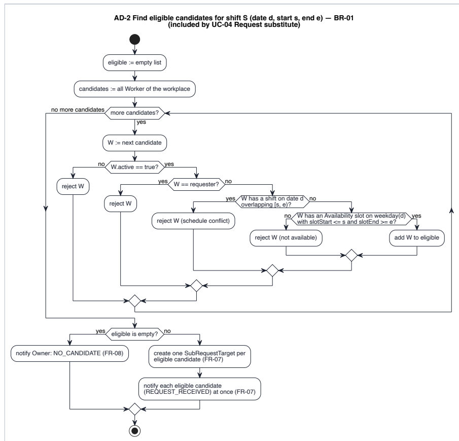
Figure 2. Activity diagram AD-2: candidate selection (BR-01)
