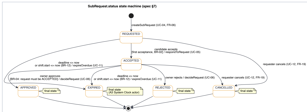
Figure 4. State machine diagram of SubRequest
