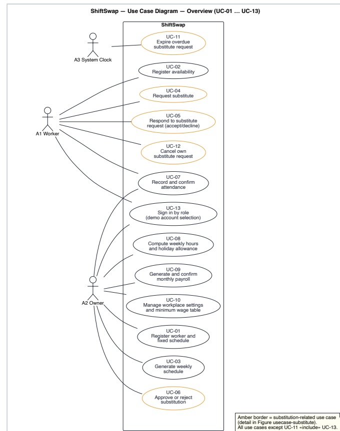
Figure 1. Use case diagram of ShiftSwap
