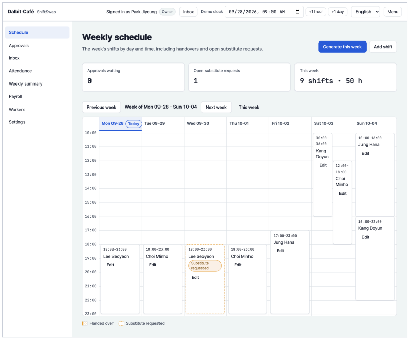
Figure 9. Weekly board, owner view (UC-03), demo clock Mon 2026-09-28 09:00. The week of Mon 09-28 to Sun 10-04 has 9 shifts and 50 h; summary cards show 0 approvals waiting and 1 open substitute request. Each shift block shows its time range, the worker and an Edit button; Generate this week and Add shift are at the top right. Lee Seoyeon's Wednesday 18:00–23:00 shift has a dashed amber outline and the chip “Substitute requested”.
