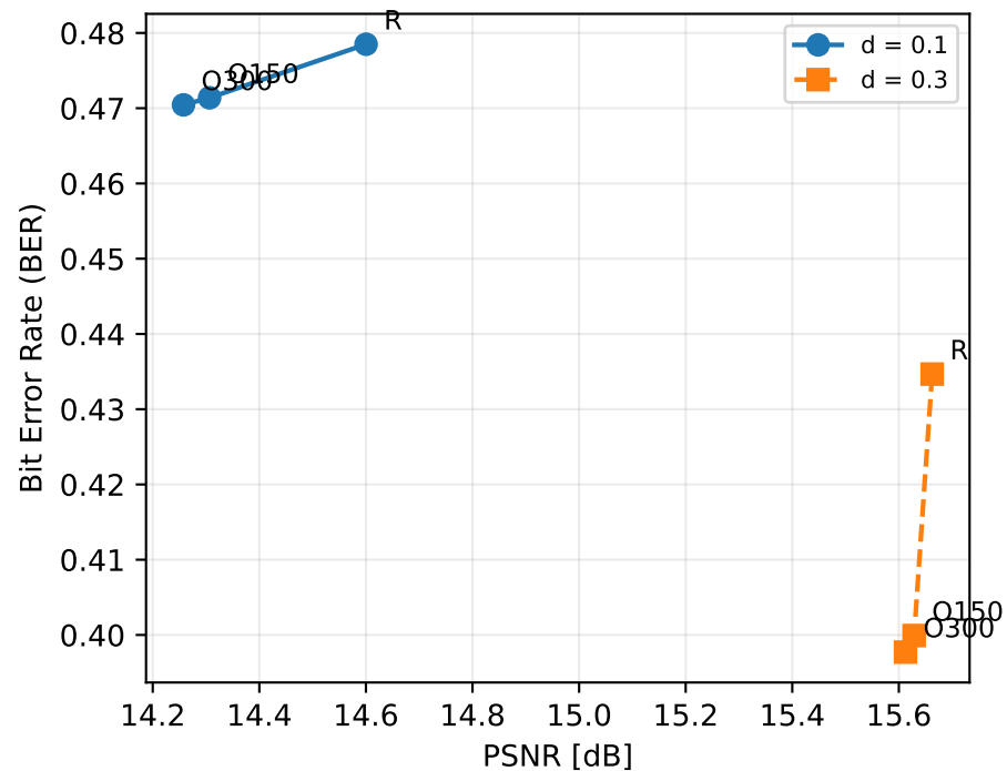
Navier-Stokes
