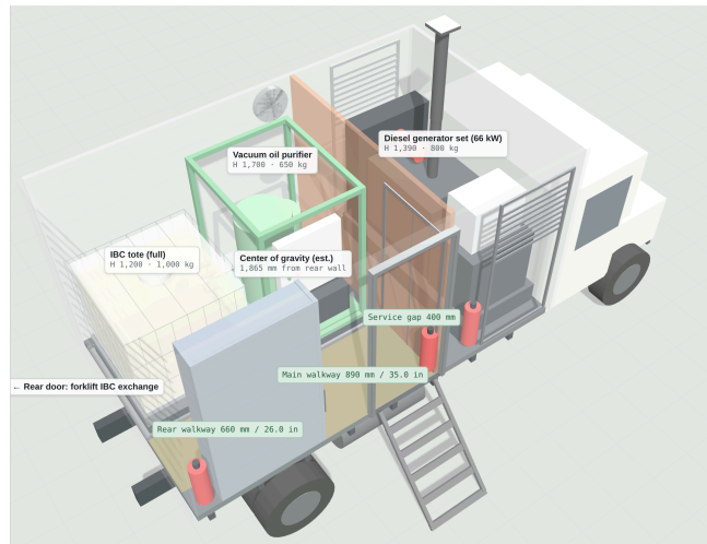
3D view of the proposed layout (interactive model attached as HTML)
