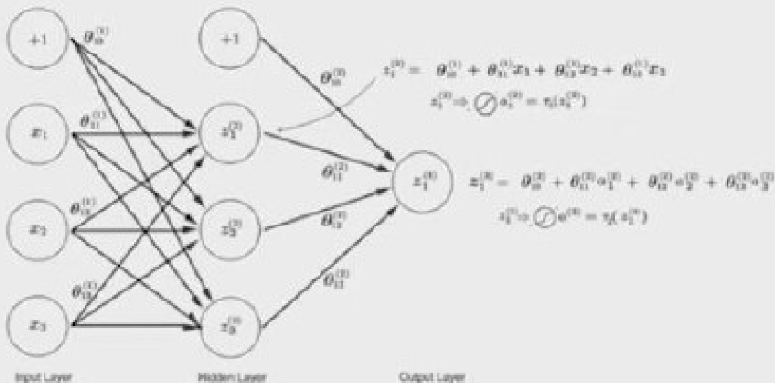
Fig 1. A neural network with one hidden layer
