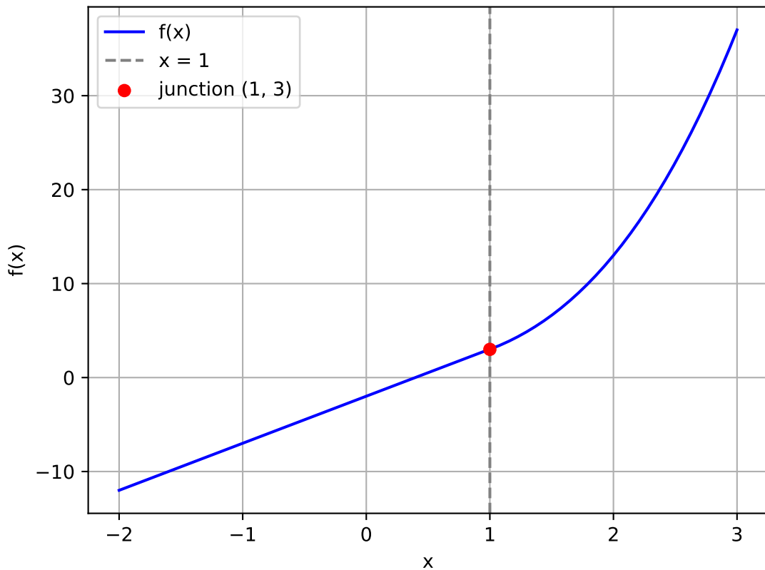
Piecewise f(x) - differentiable at x = 1
