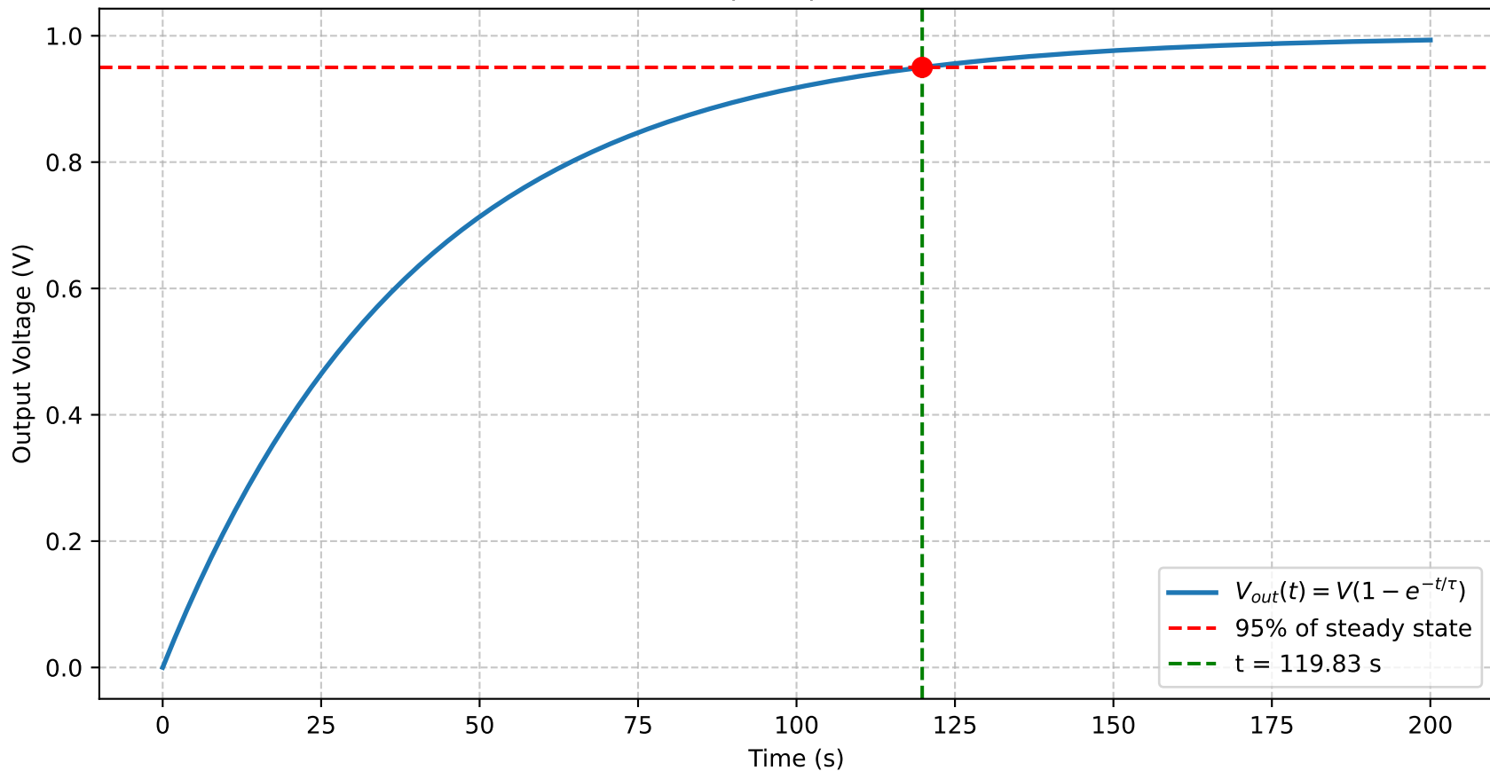
First-Order Step Response ( \tau = 40.0 s)
