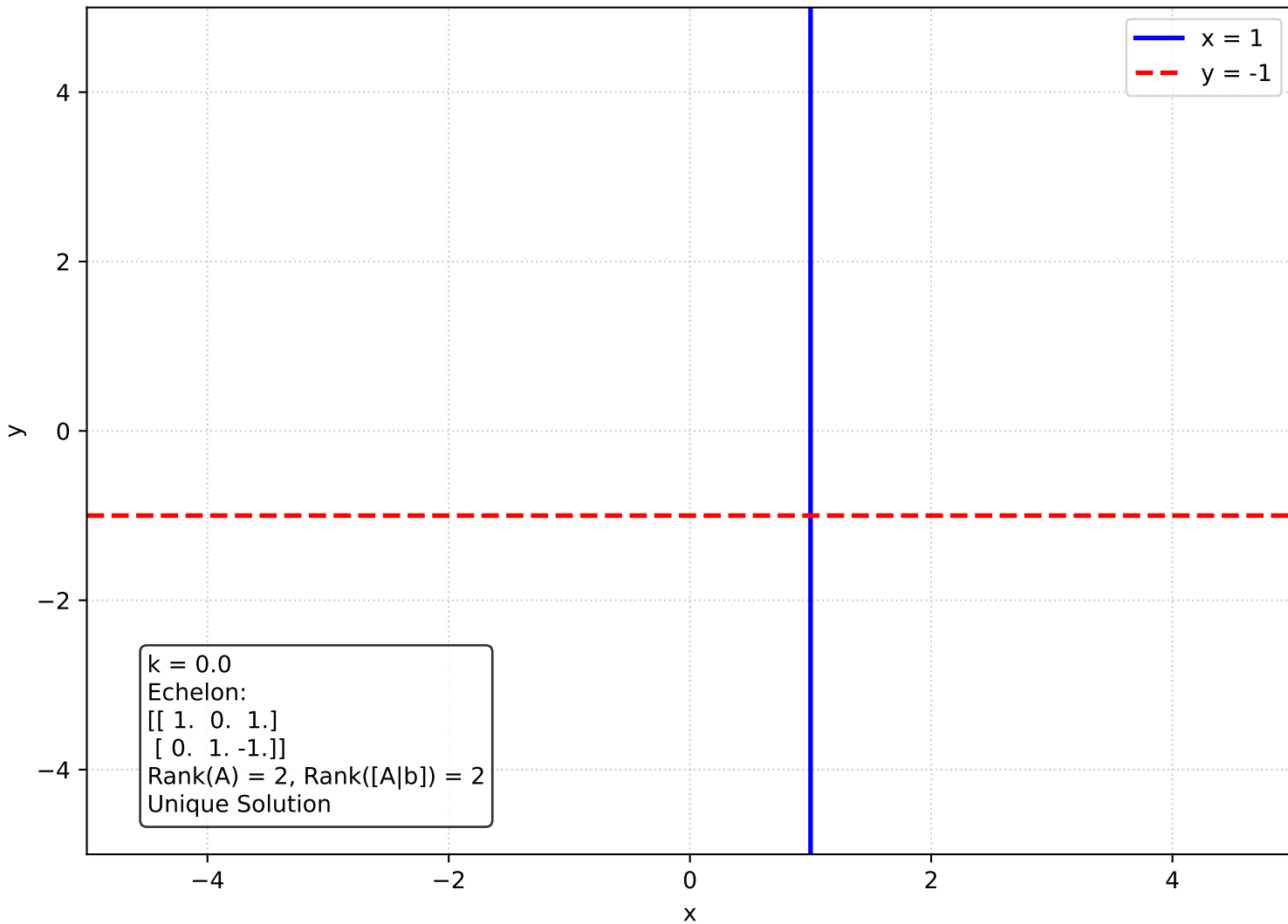
Graph for k = 0.0 (Unique Solution)
