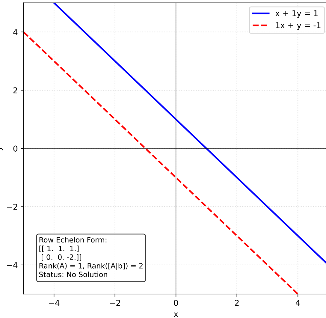
No Solution (k = 1)
