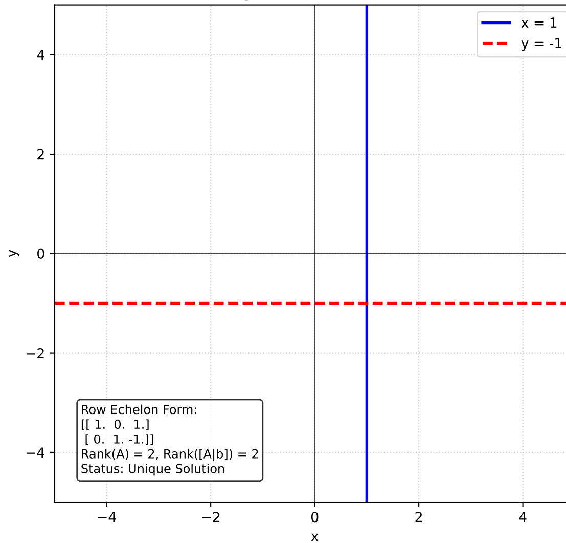
Unique Solution (k = 0)
