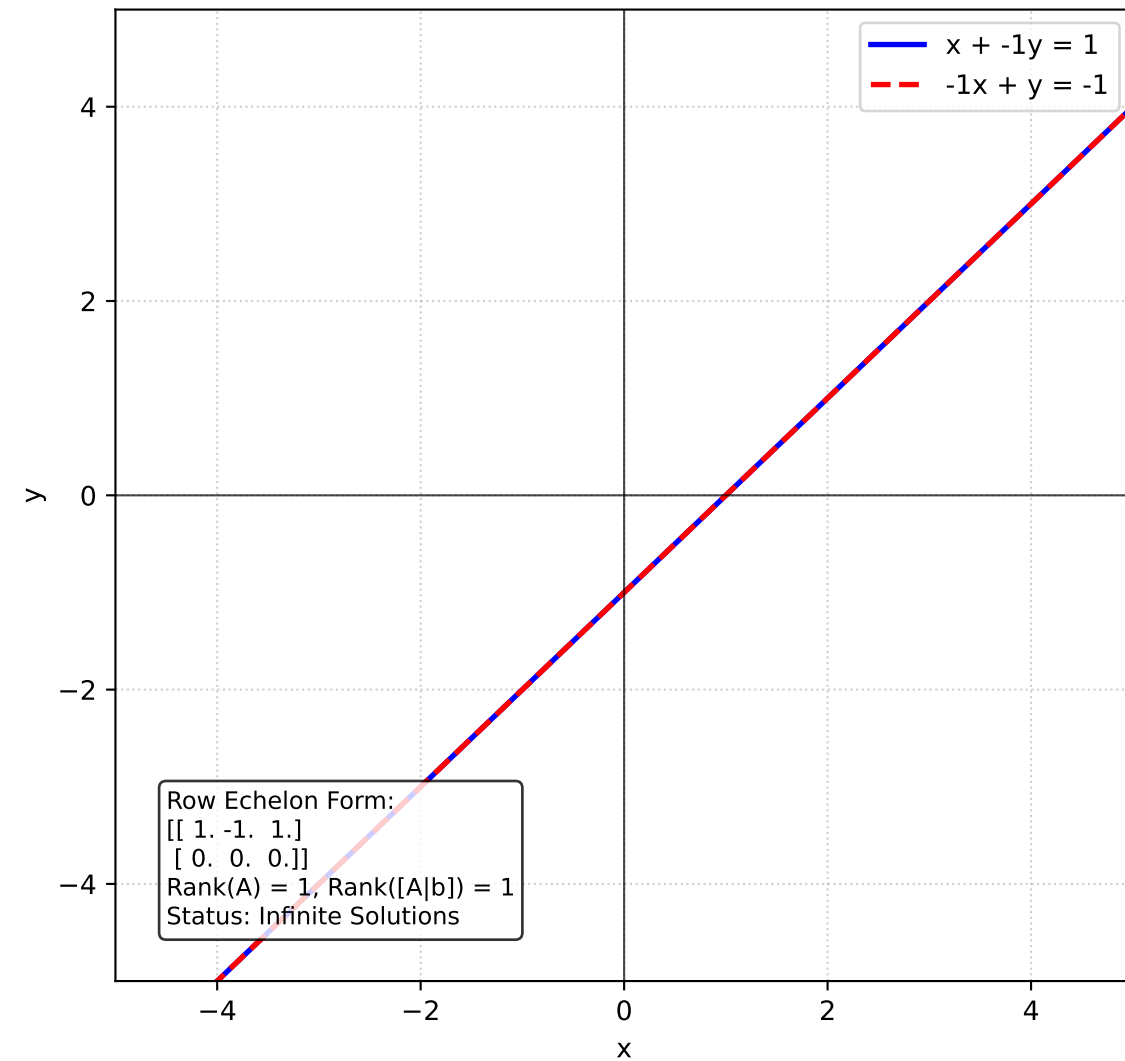
Infinite Solutions (k = -1)
