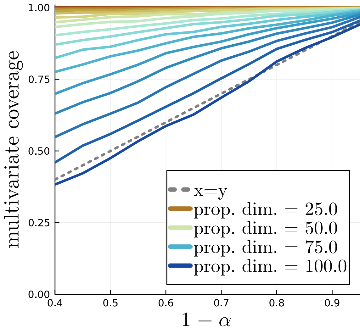
(b) multi-conformal: \rho = 0.3
