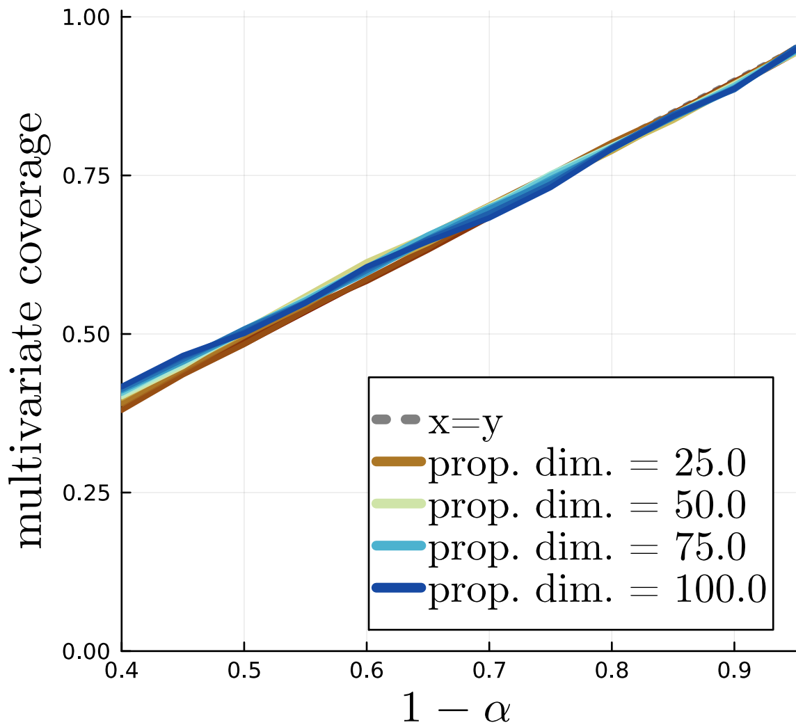
(b) prop-multi-conformal
