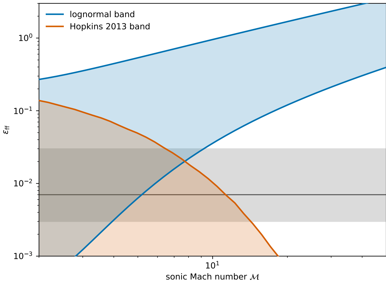
KM05 envelope ( b = 1/3 \rightarrow 1 ): lognormal vs Hopkins PDF
