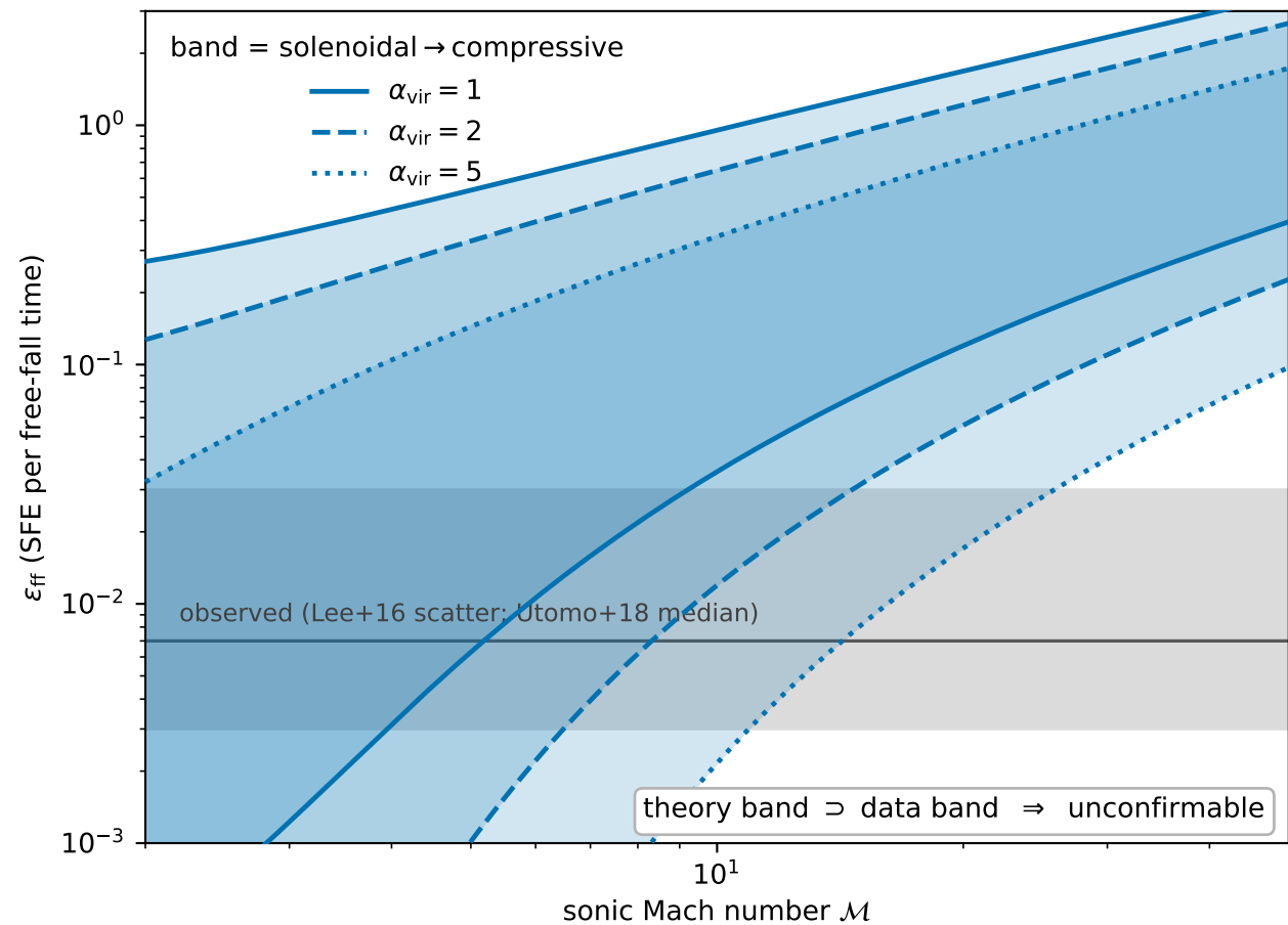
KM05 multi-ff: driving-parameter envelope ( b = 1/3 \rightarrow 1 ) vs data
