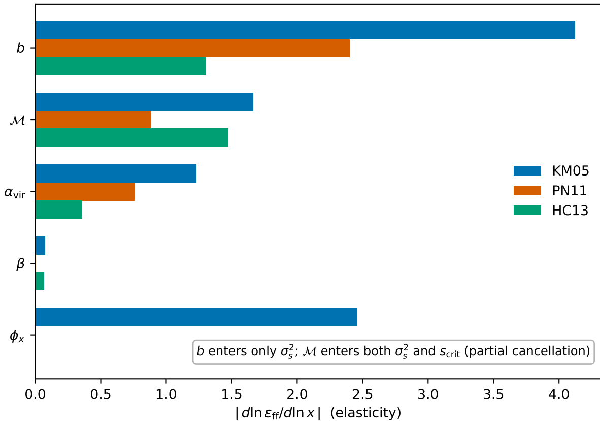
Parameter leverage at fiducial ( b = 0.4 , \mathcal{M} = 10 , \alpha_{\text{vir}} = 1 , \beta = 10 )
