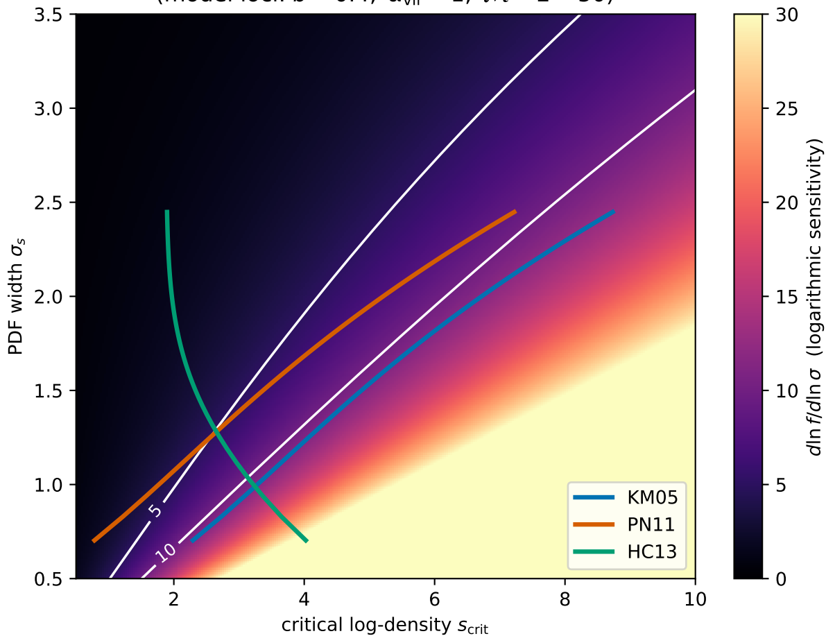
Sensitivity of the mass fraction to \sigma_s (model loci: b = 0.4 , \alpha_{\text{vir}} = 1 , \mathcal{M} = 2 \rightarrow 50 )
