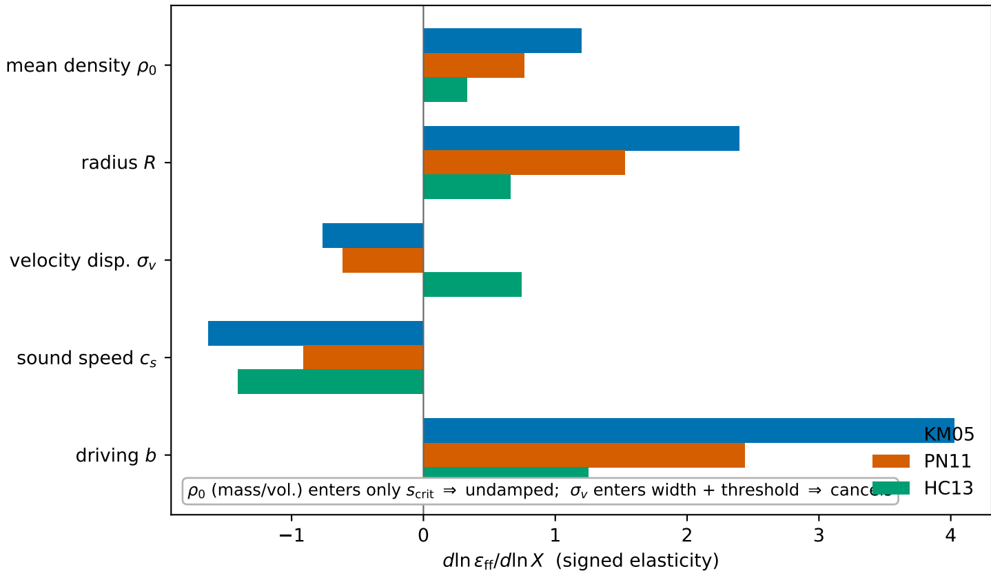
Sensitivity of \varepsilon_{\text{ff}} to physical observables (fiducial b = 0.4 , \mathcal{M} = 10 , \alpha_{\text{vir}} = 1 )
