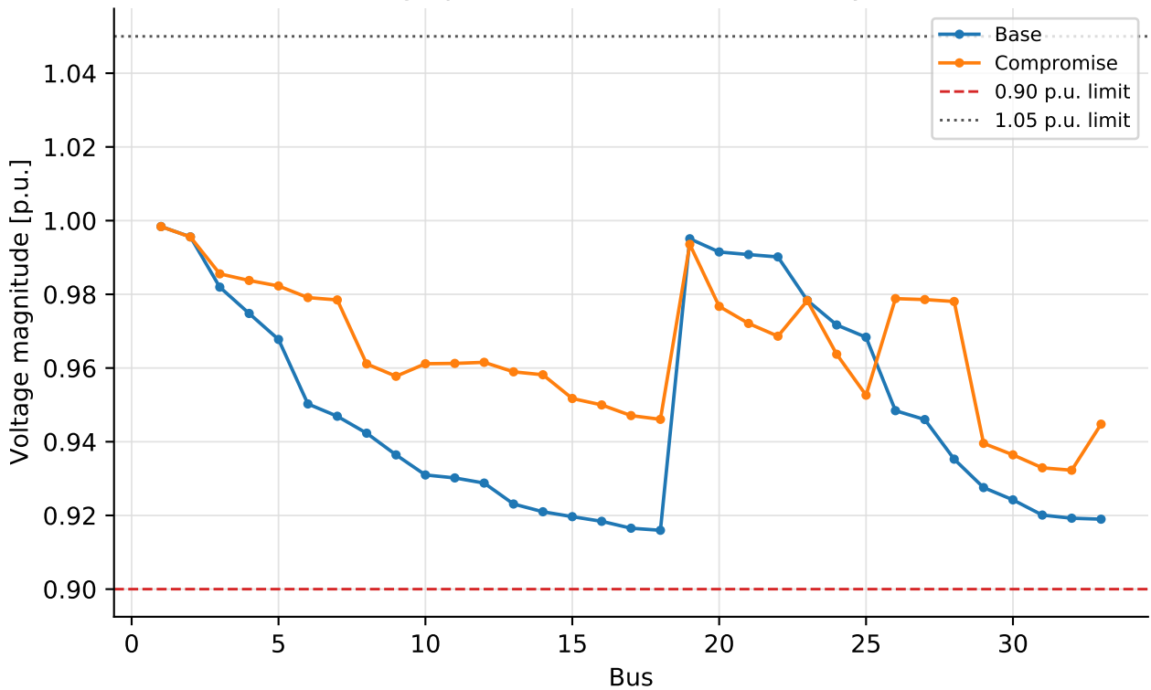
Voltage profile for the IEEE 33-bus system
