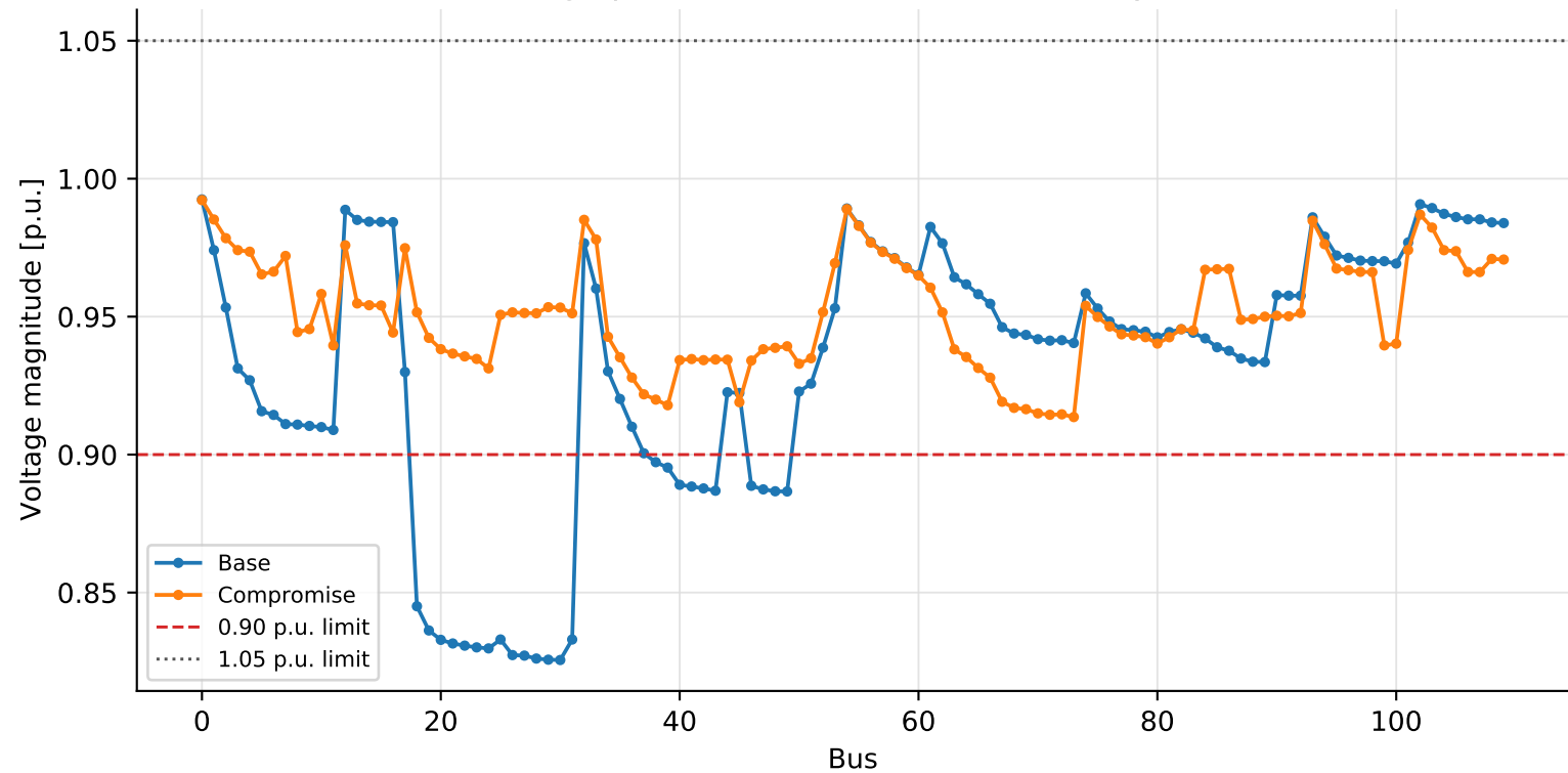
Voltage profile for the real distribution system
