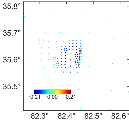
S1_T158A_ifg Data
