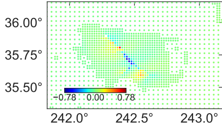
Residuals
