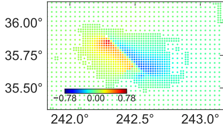
Model
