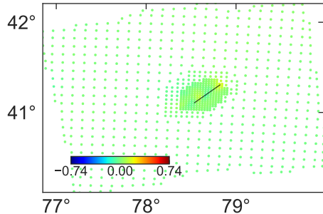
Residuals
