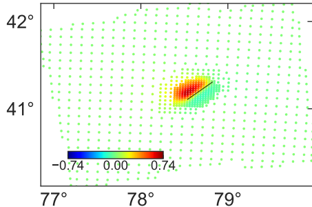
Model
