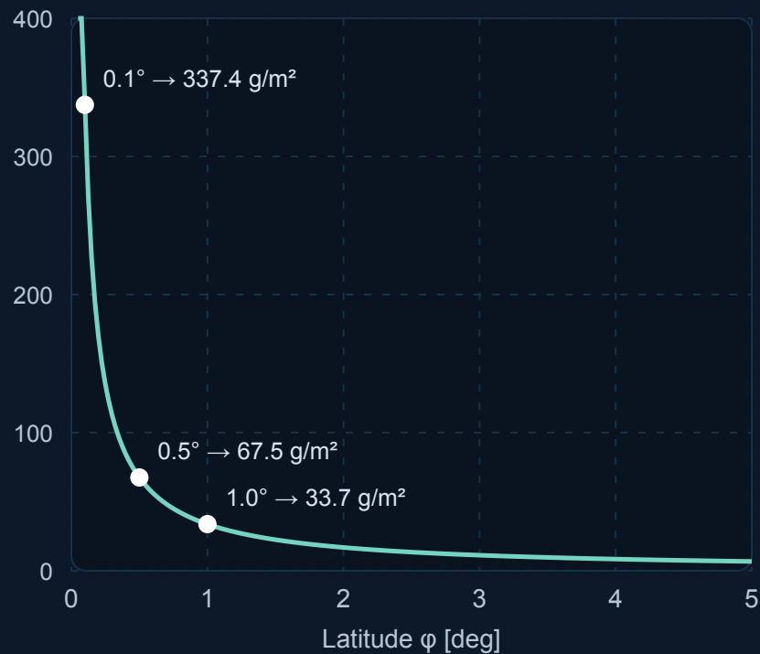
Max areal density \sigma_{\max}(\varphi) [g/m 2 ]
