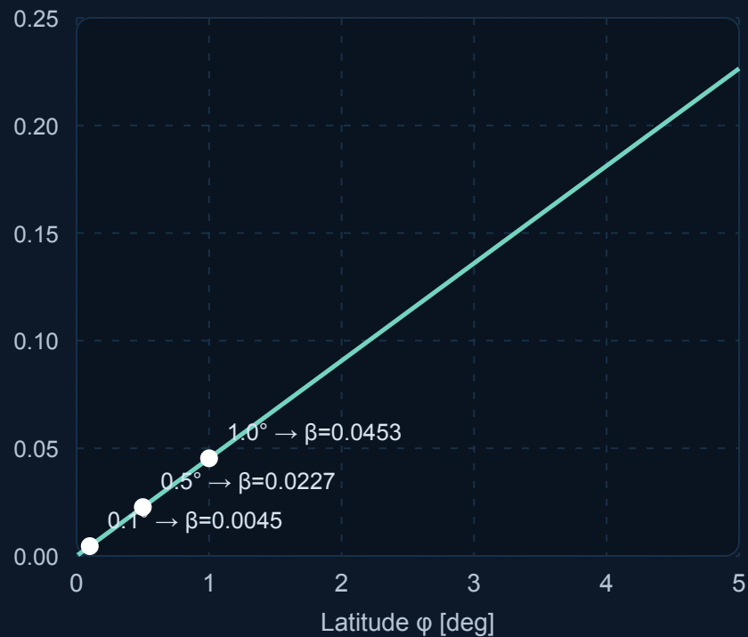
Required lightness number \beta_{\min}(\varphi)
