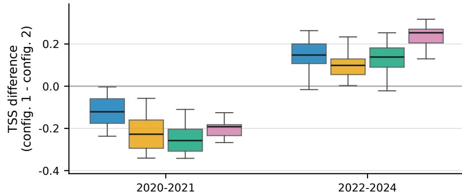
b F1: Logreg-O-DEF - Logreg-O-NRT
