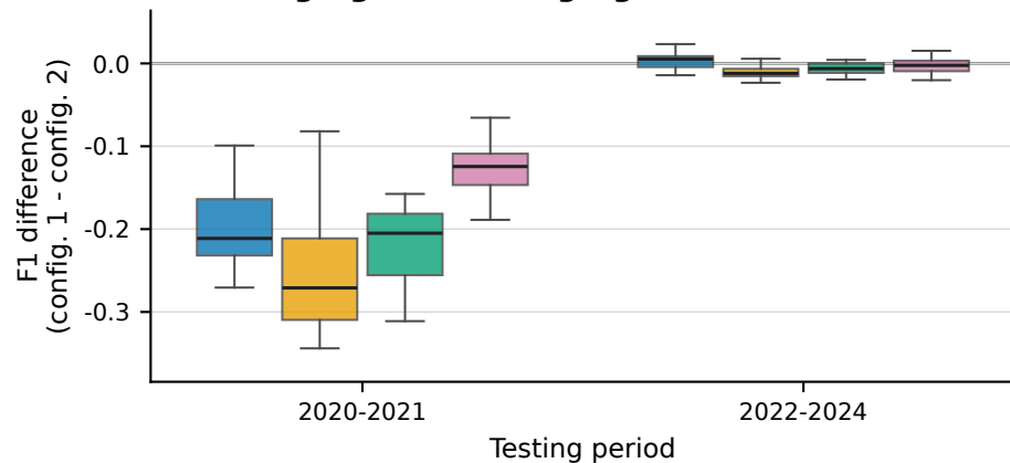
b F1: Logreg-O-DEF - Logreg-O-NRT
