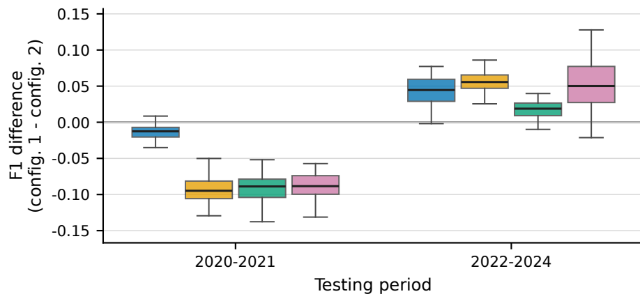
b F1: LSTM-S-DEF - LSTM-O-DEF
