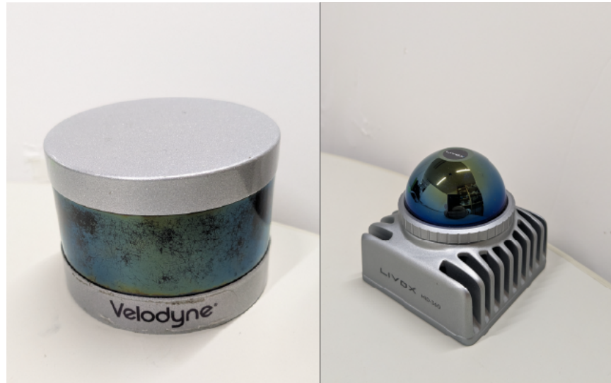
図 1.3 3D LiDAR (Left: Velodyne, Right: Livox)
