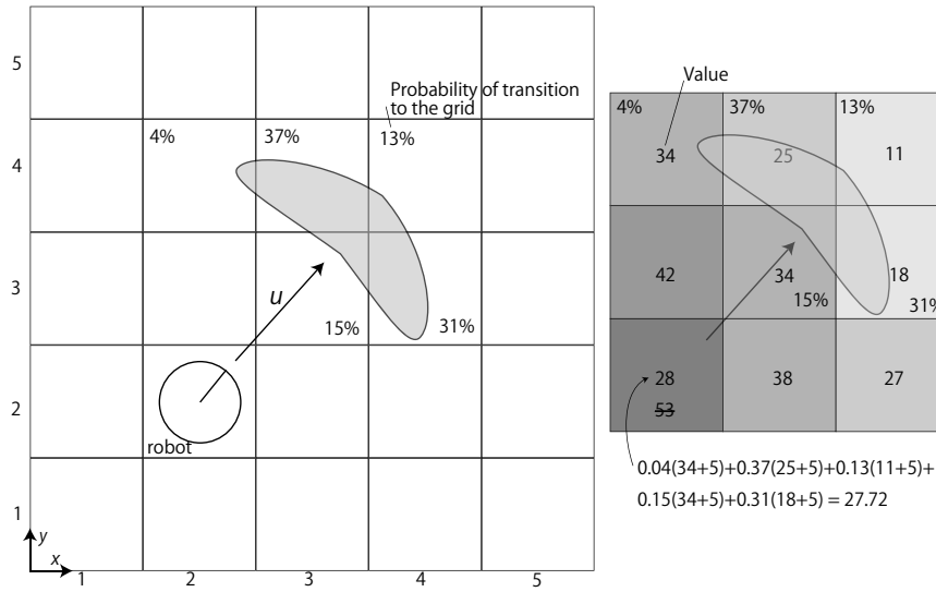
図 2.2 Calculation of the state value function
