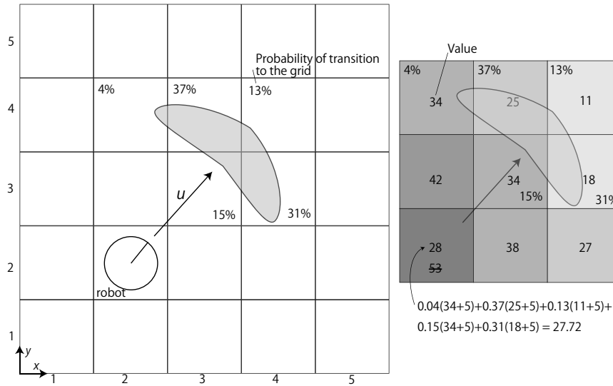
図 2.2 Calculation of the state value function
