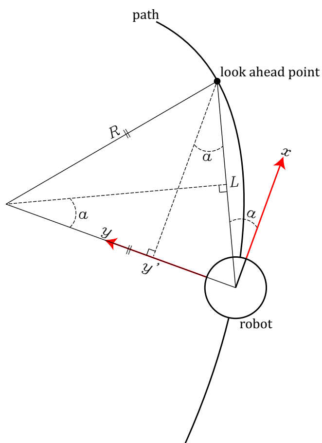
☒ A.1 how follow the path by pure pursuit
