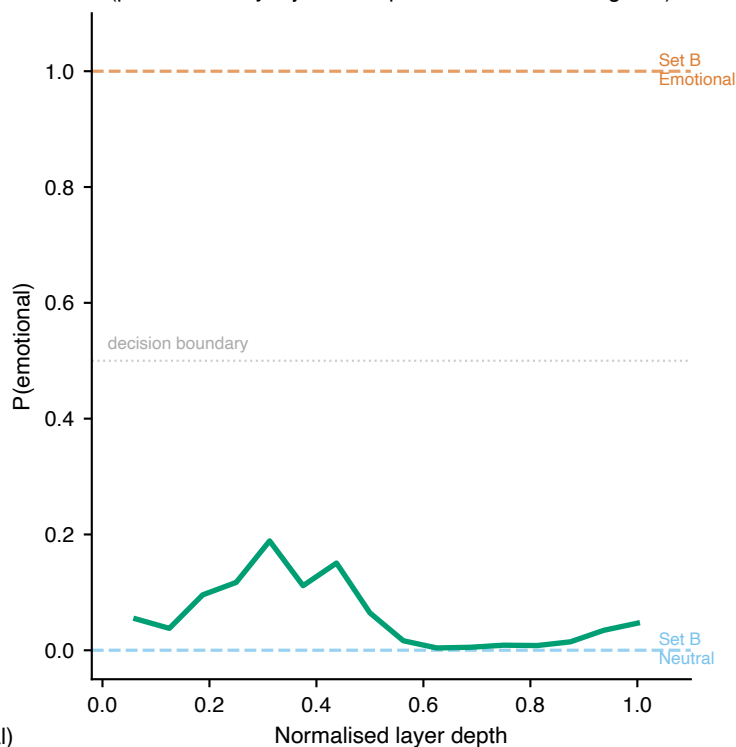
B — Set C probe trajectory across layers (probe correctly rejects complex-neutral text throughout)
