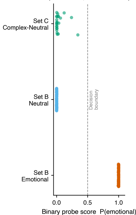
A — Probe score distributions (0 = neutral, 1 = emotional)
