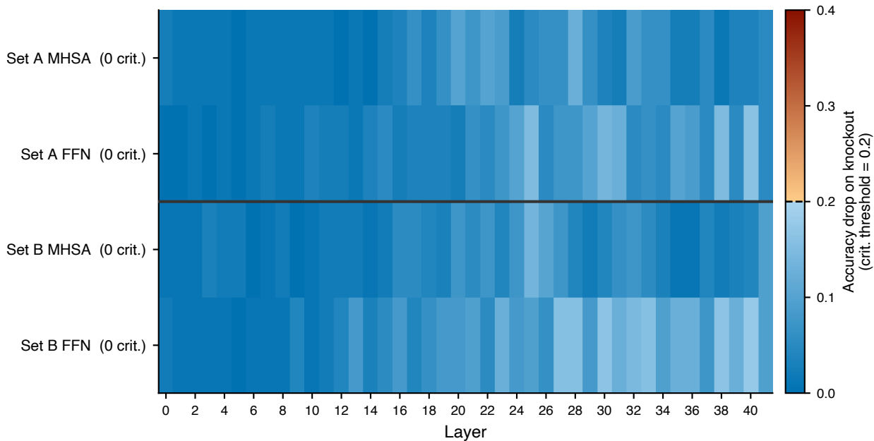
Knockout fragility: Gemma9B Inst (zero-ablation; Set A = keyword-rich, Set B = clinical)
