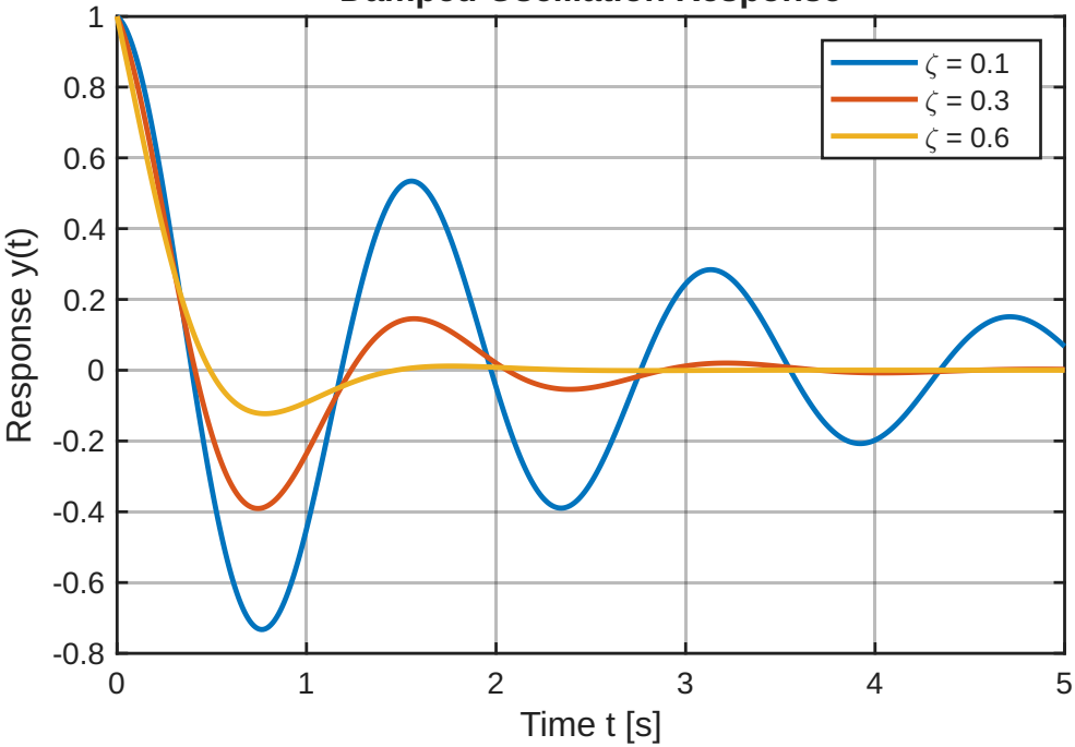
Damped Oscillation Response
