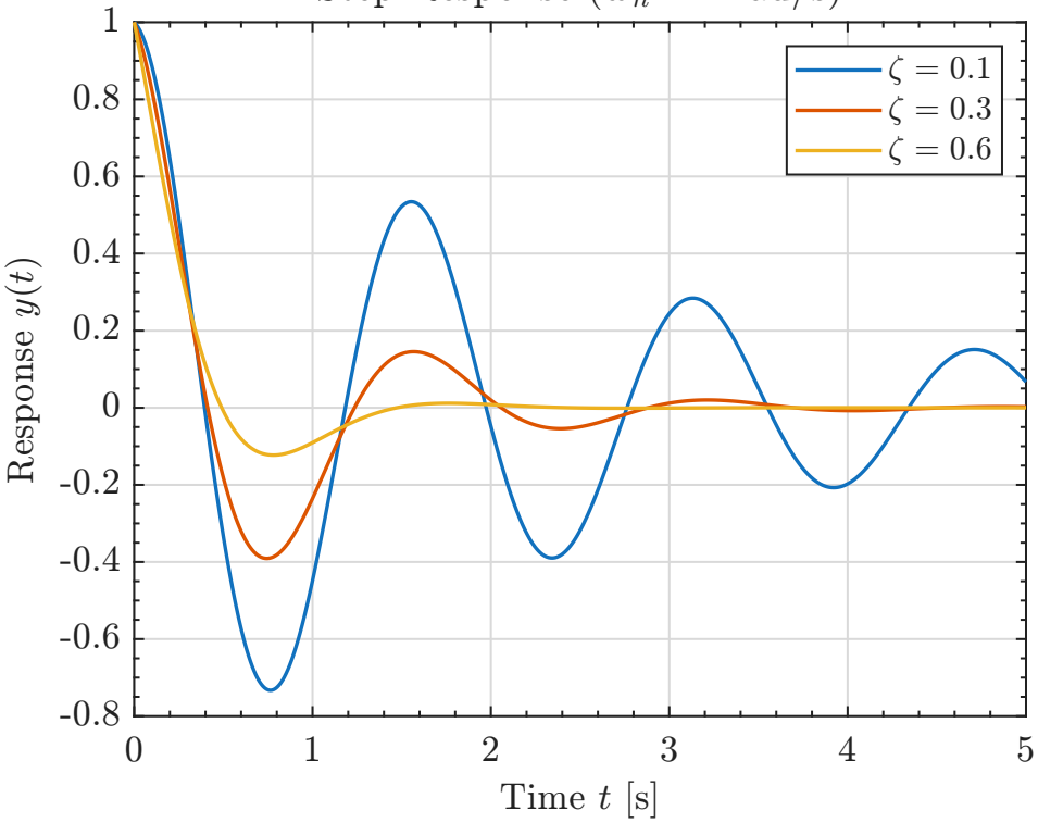
Step Response ( w_n = 4 \text{ rad/s} )
