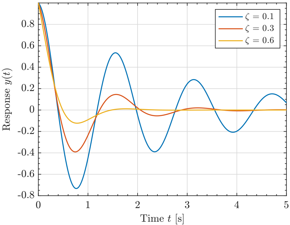
Step Response ( \omega_n = 4 \text{ rad/s} )
