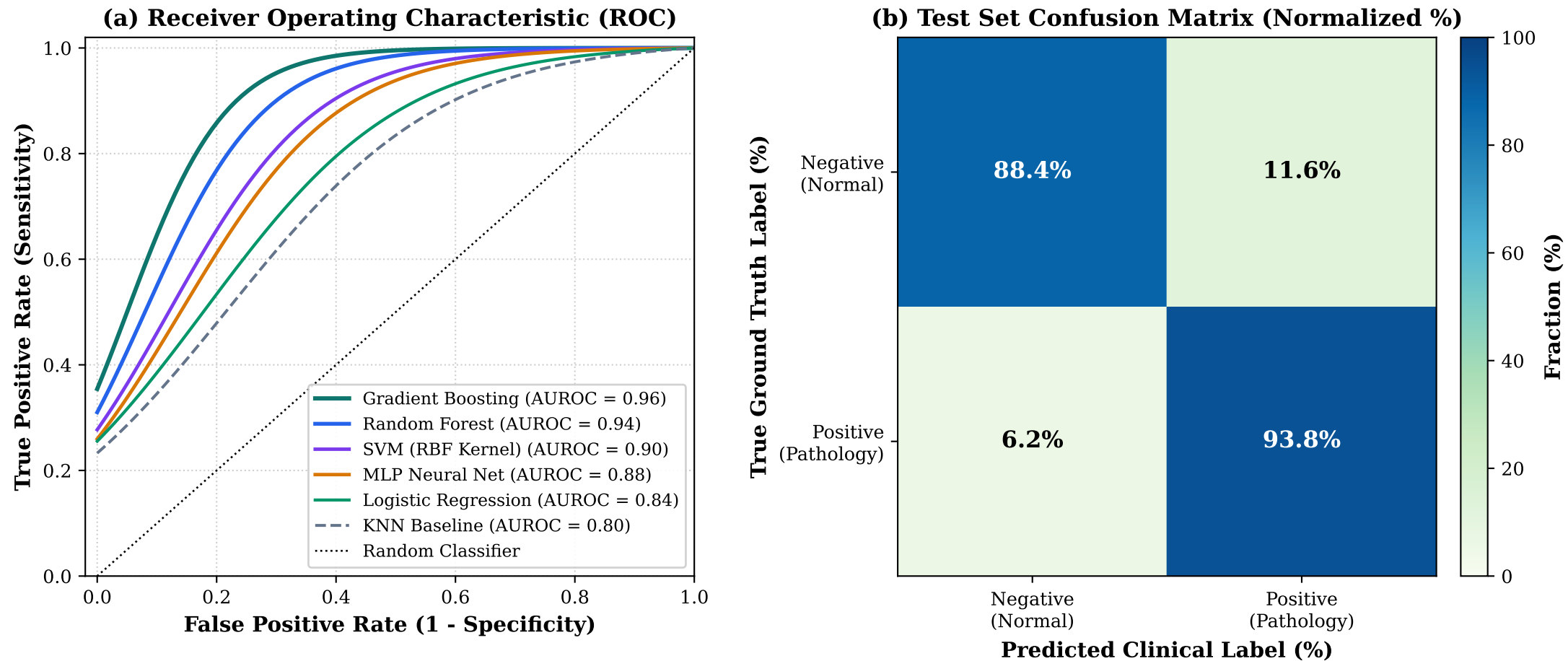
Fig. 3. Multi-Model Discriminative Capacity and Clinical Decision Trade-offs
