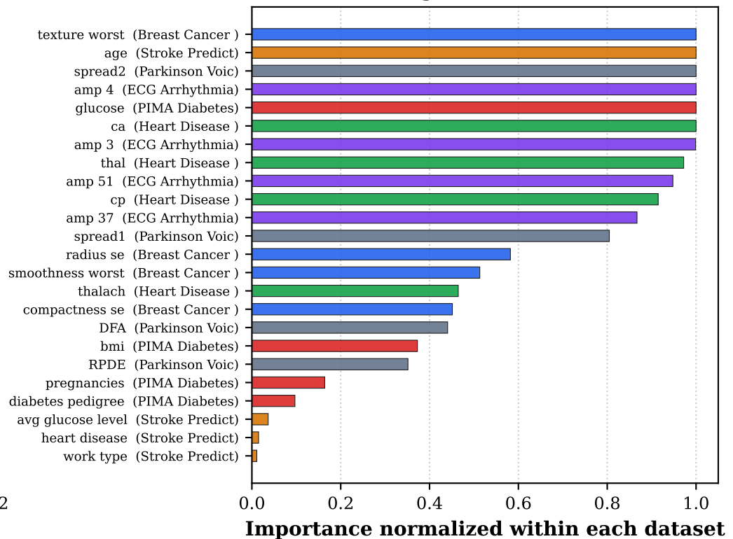
(b) Top-ranked inputs of the tabular and signal cohorts
