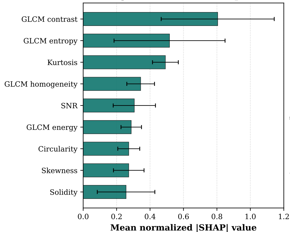
(a) Radiomic descriptors, averaged over the 4 image collections (TreeExplainer)
