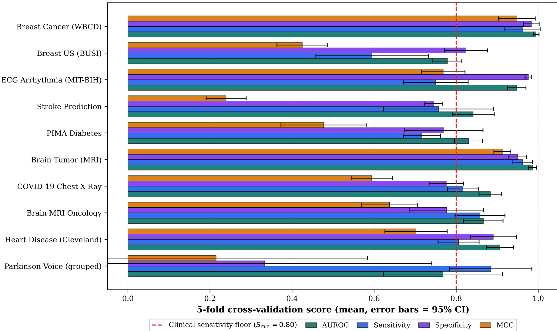
Performance of the clinically selected model on ten real biomedical datasets
