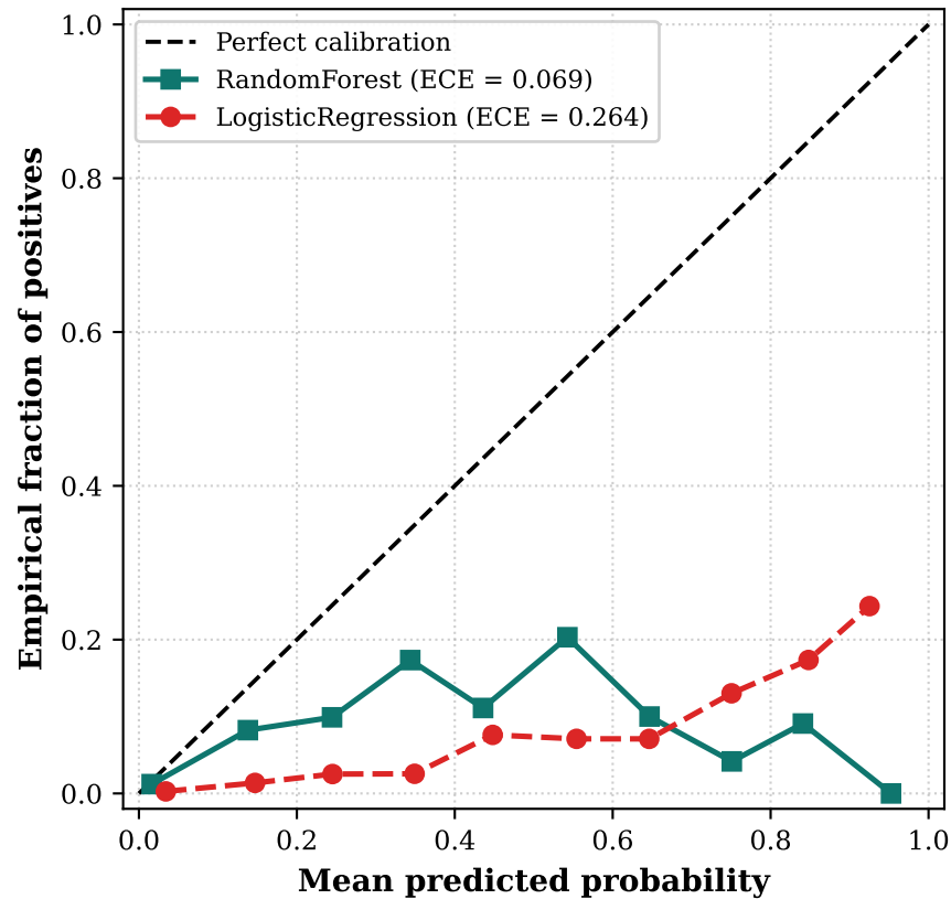
(a) Reliability diagram - Stroke Prediction (out-of-fold) (b) Calibration of the selected model per dataset
