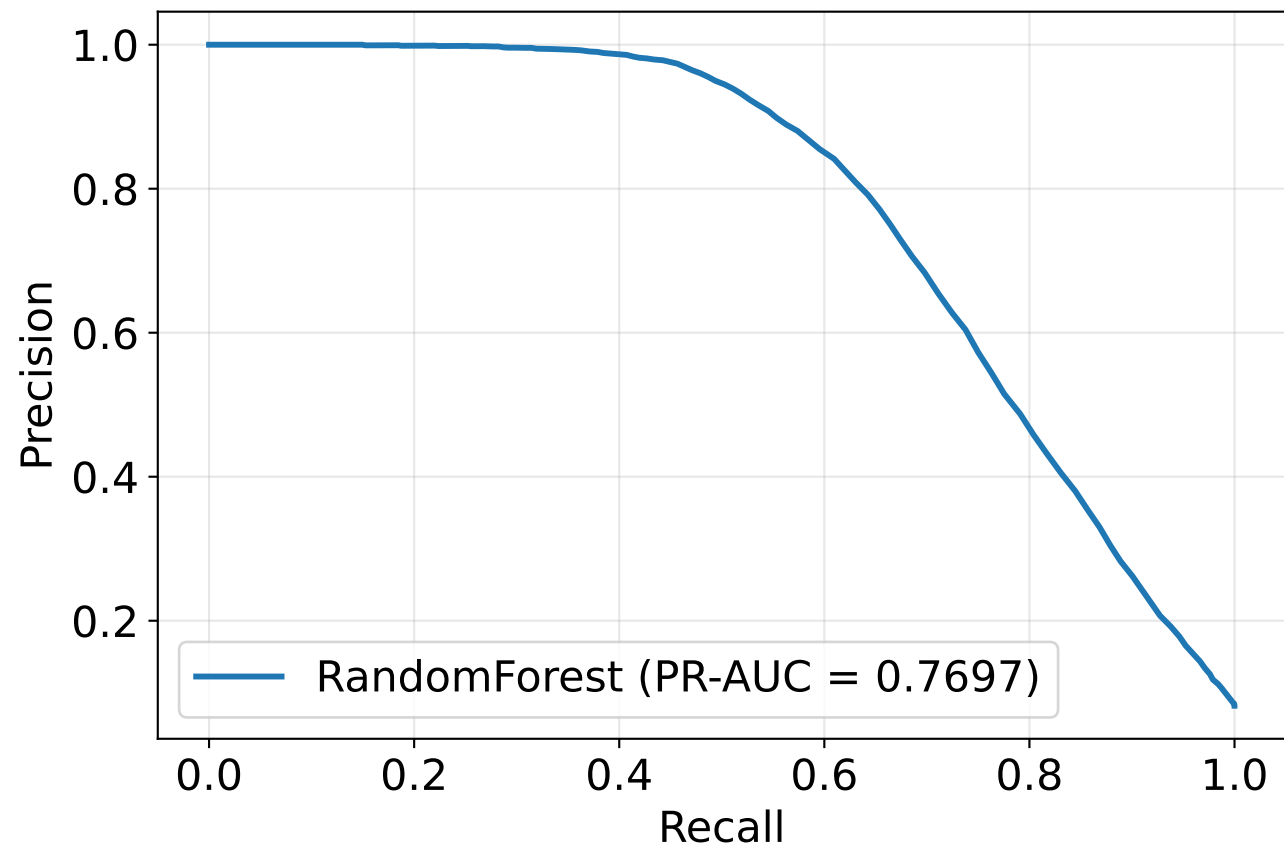
Precision-Recall Curve - Best Baseline Model
