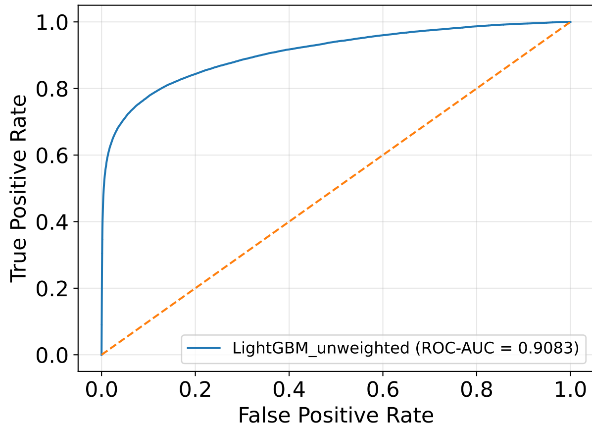
ROC Curve - Test 2025
