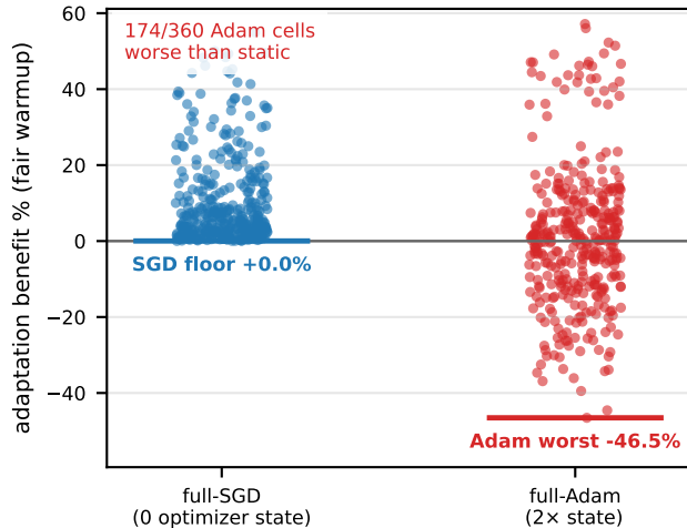
(B) SGD floor vs Adam negative tail
