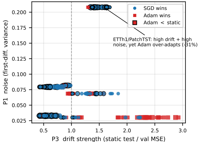
(A) which optimizer wins, drift \times noise
