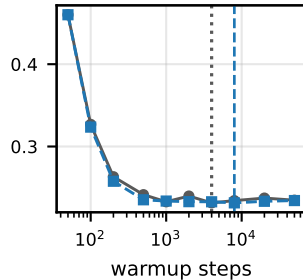
Appliances / DLinear
