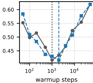
Appliances / PatchTST
