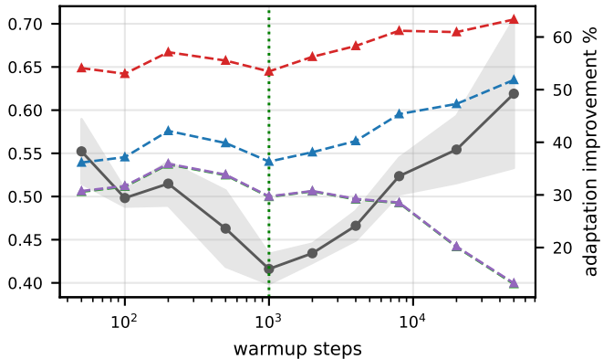
Appliances / PatchTST
