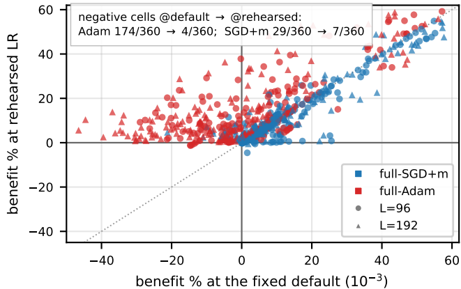
(B) rehearsal rescues Adam; can sink SGD (bottom edge)
