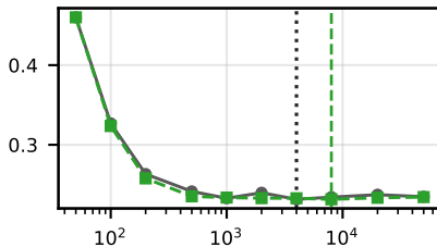
Appliances / DLinear
