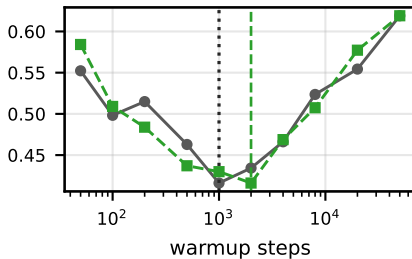
Appliances / PatchTST
