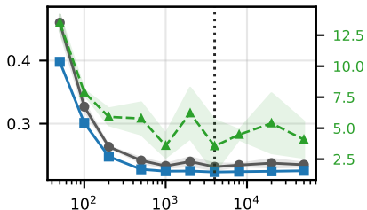
Appliances / DLinear
