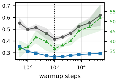
Appliances / PatchTST
