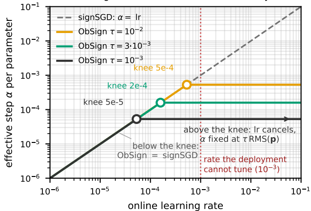
(A) the effective step \alpha = \min(\text{lr}, \tau \text{RMS}(\mathbf{p})) has two regimes, and the knee is where they meet
